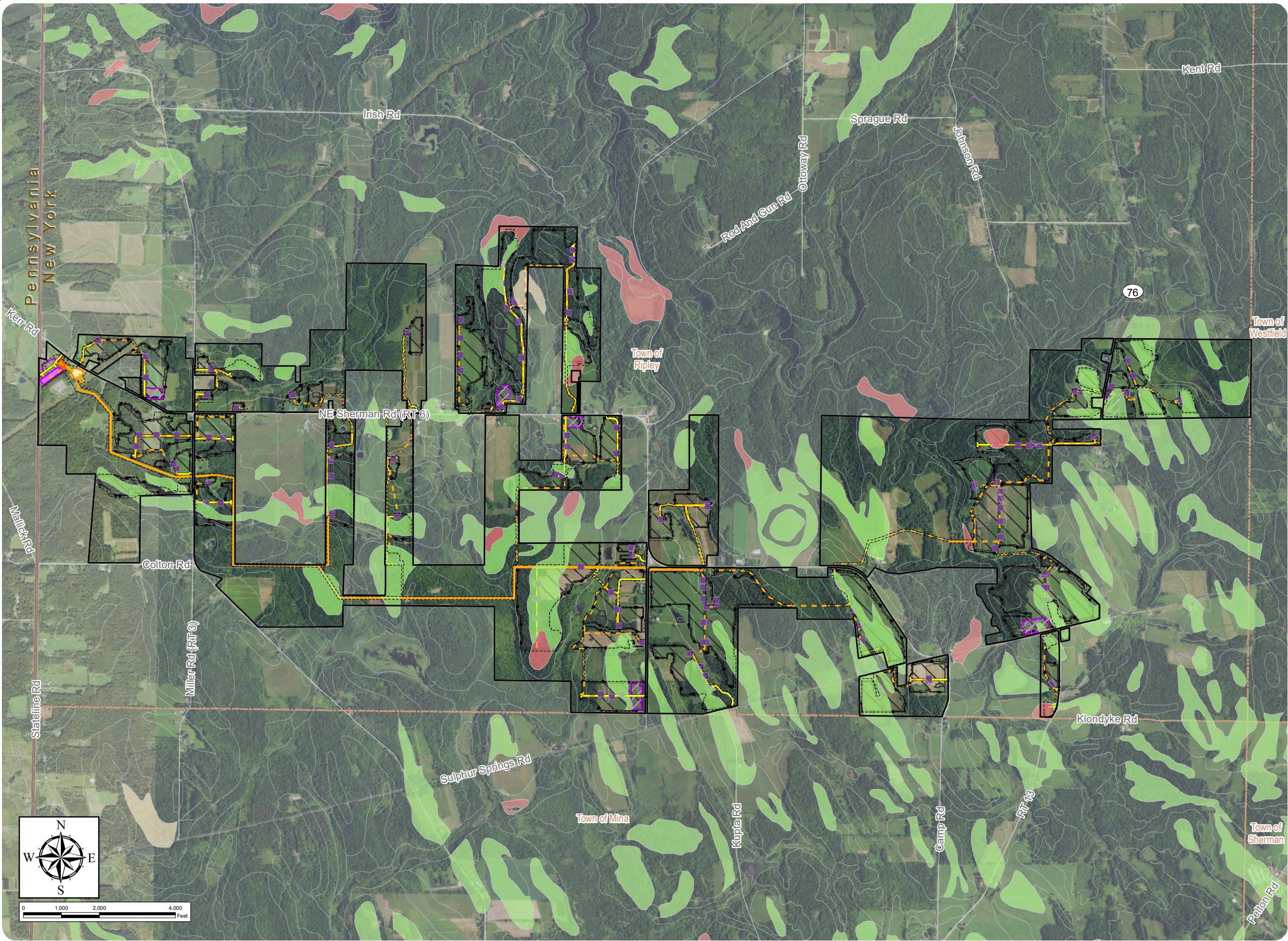
Figure S15-6: Mineral Soil Groups
