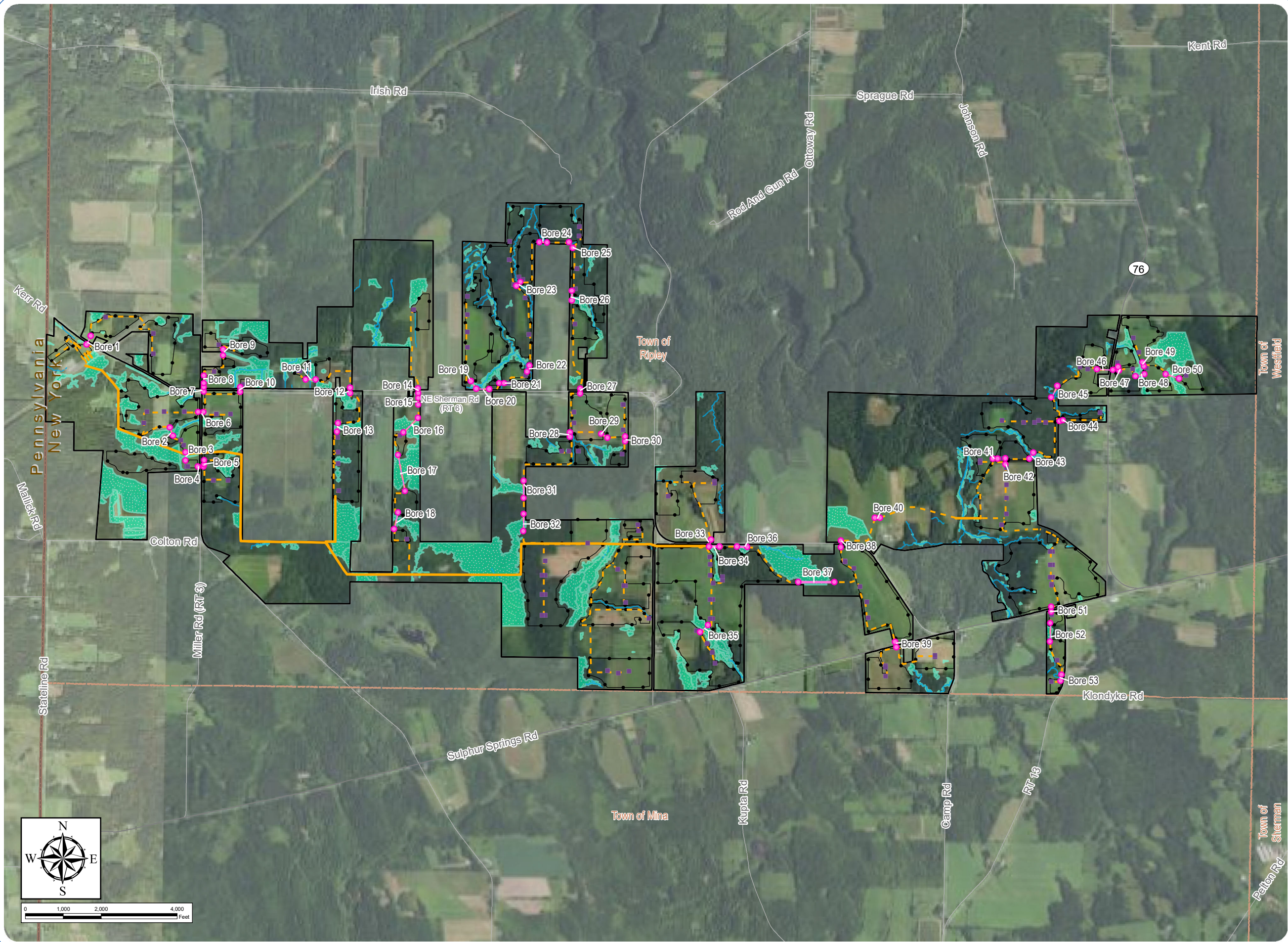
Figure S10-2: Trenchless Installation Locations
